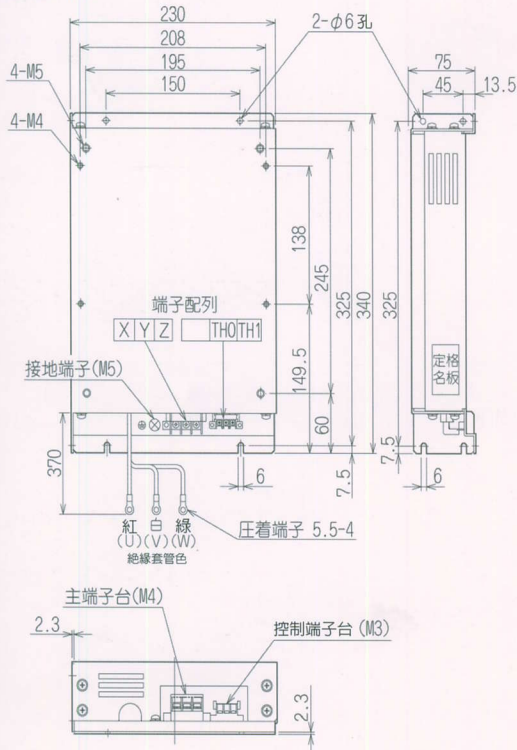
● FR-BMF-H7.5K
