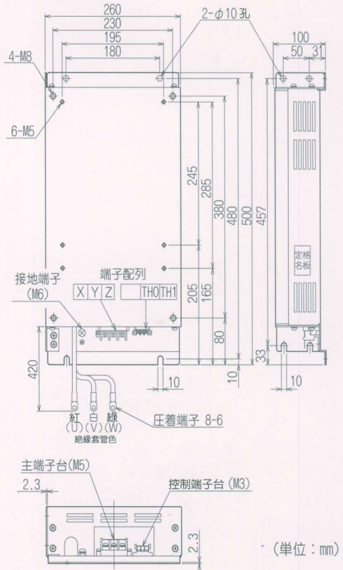
● FR-BMF-H15K
