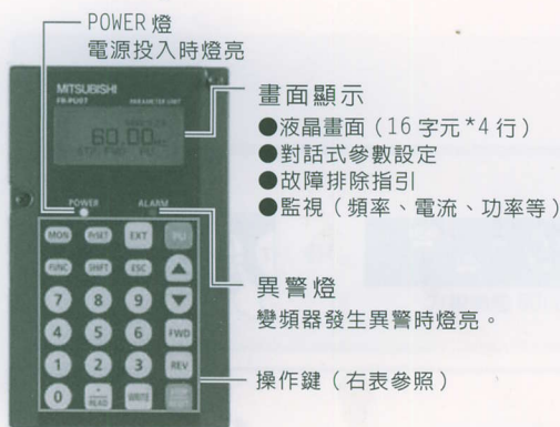
FR-PU07
